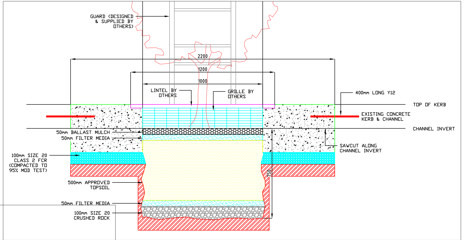
ROADSIDE ELEVATION 1:100
