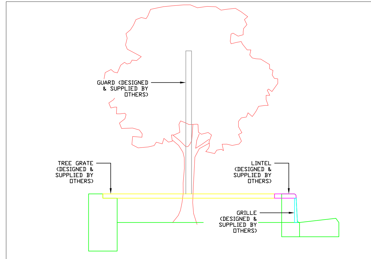
ROADSIDE ELEVATION 1:100
